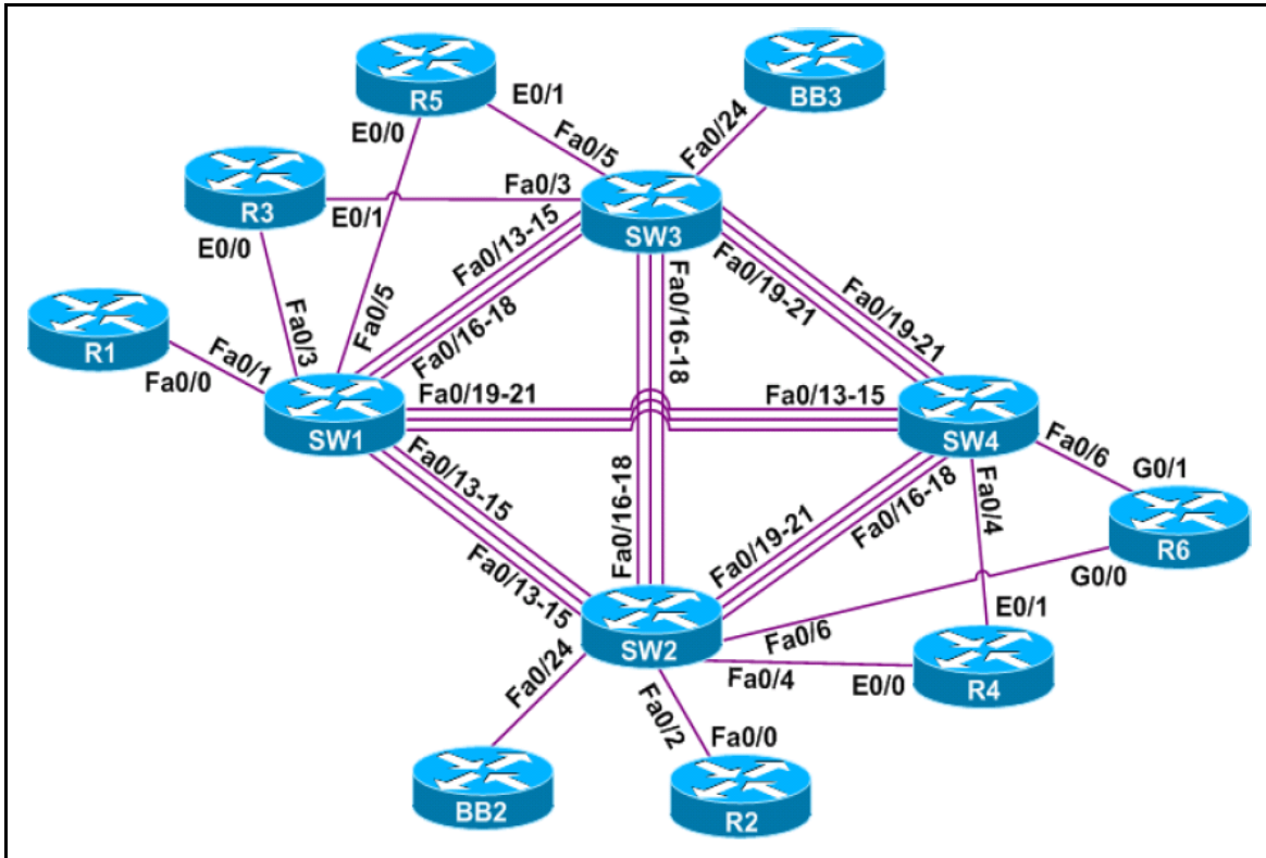
R&S Lab Rack Physical LAN Cabling
